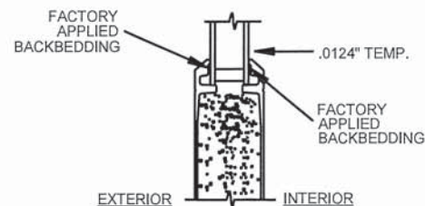
TYPICAL GLAZING DETAIL NON-IMPACT GLASS
